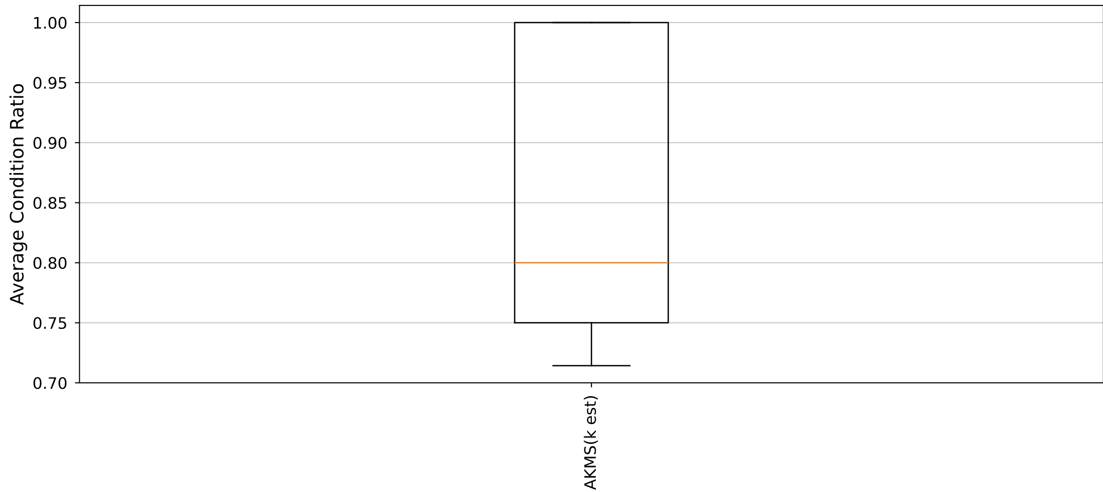
YARA Rules Average Condition Ratio Distribution (Cluster34_Size5 dataset)
